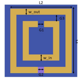
Fig. 3. Unit cell's substrate (blue) and S-SRR (yellow).
